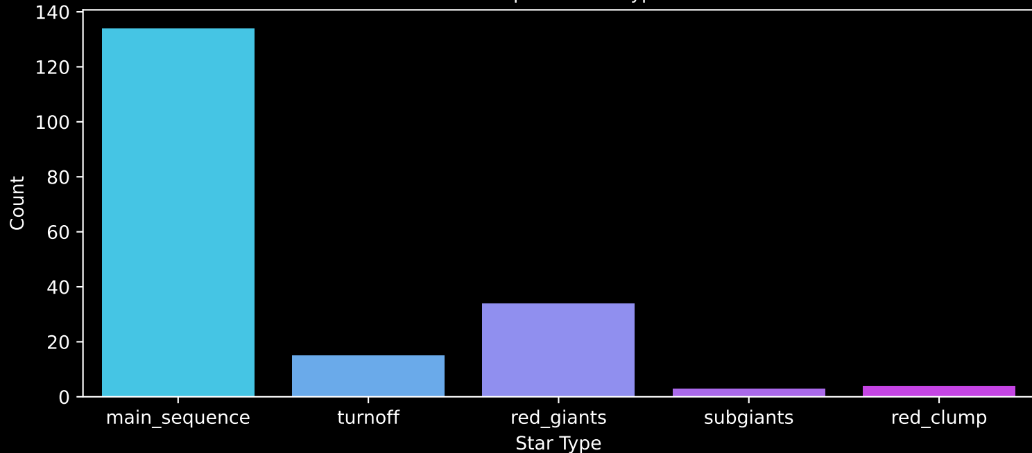
APOGEE DR17 Field: [K2_C8_124-63_btx] Count plot of Star Type
