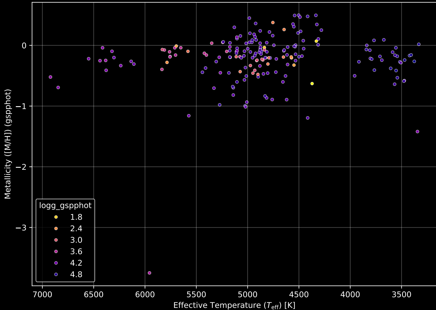
APOGEE DR17 Field: [K2_C8_124-63_btx] Stellar Population Parameters (n= 190)
