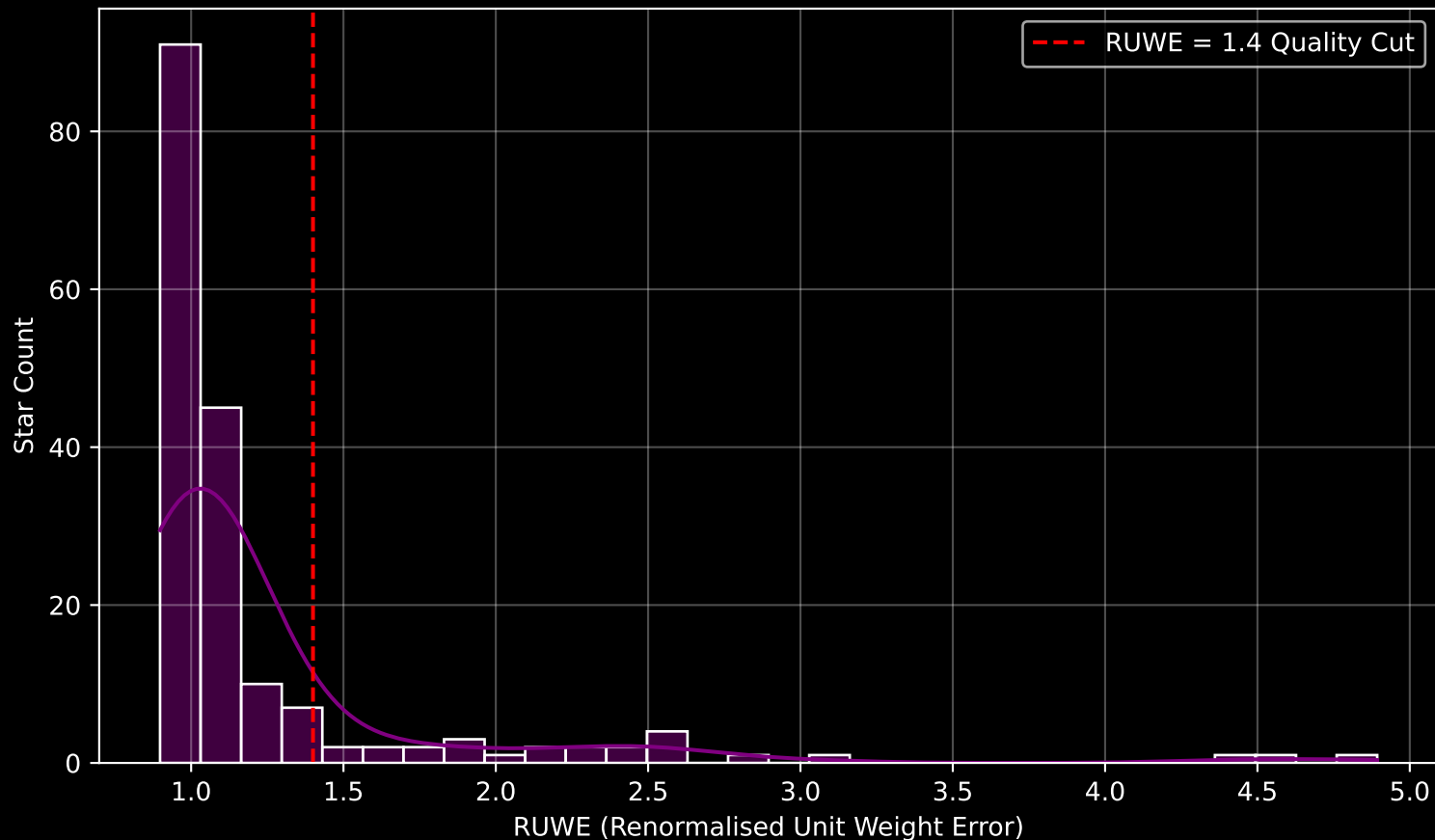
GAPOGEE DR17 Field [K2_C8_124-63_btx] RUWE Distribution (n= 178)
