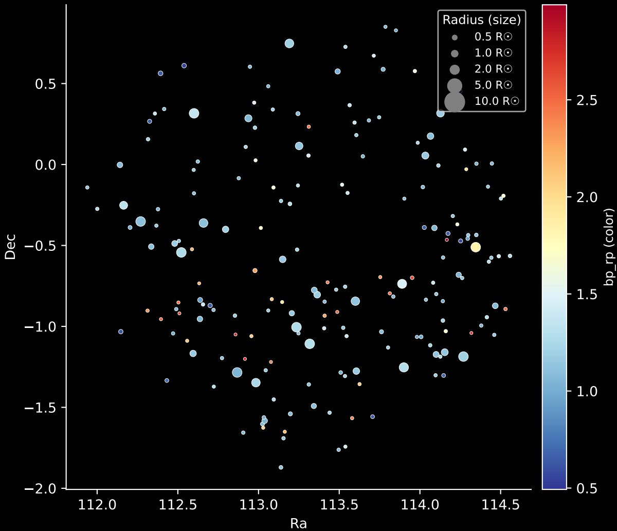
APOGEE DR17 Field: [K2_C8_124-63_btx] Stars: 190
