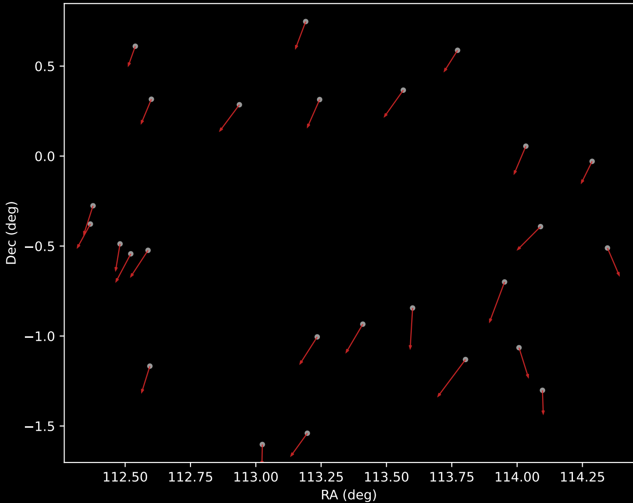
APOGEE DR17 Cluster 6 Proper Motion Vectors (n=26)
