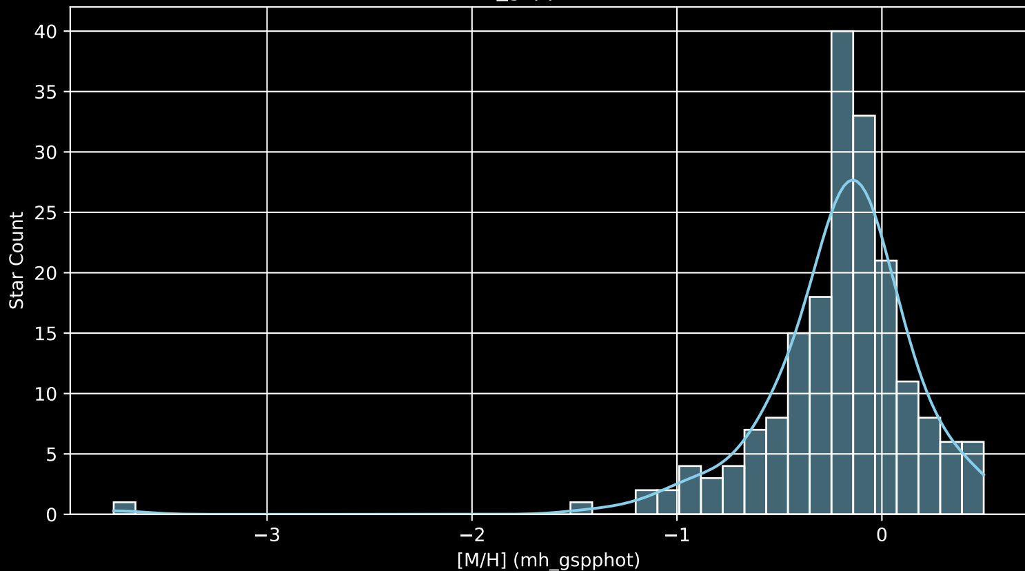
APOGEE DR17 Field: [K2_C8_124-63_btx [M/H] (mh_gspphot) (n= 190)
