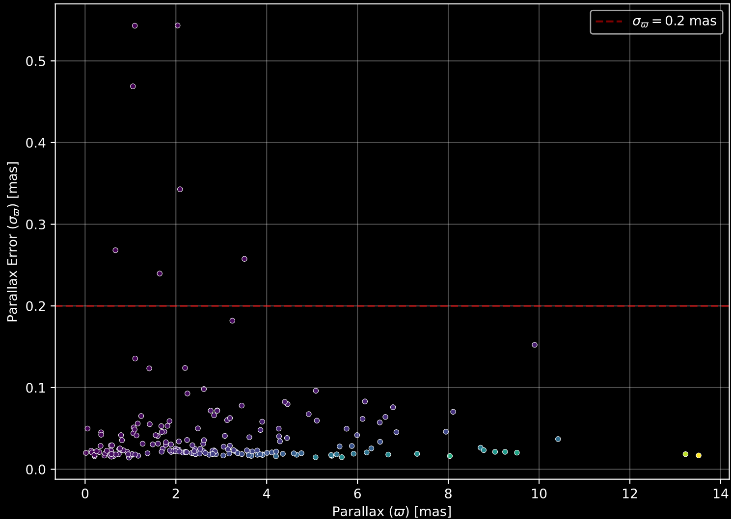
APOGEE DR17 Field: [K2_C8_124-63_btx] Parallax Quality (n= 190)
