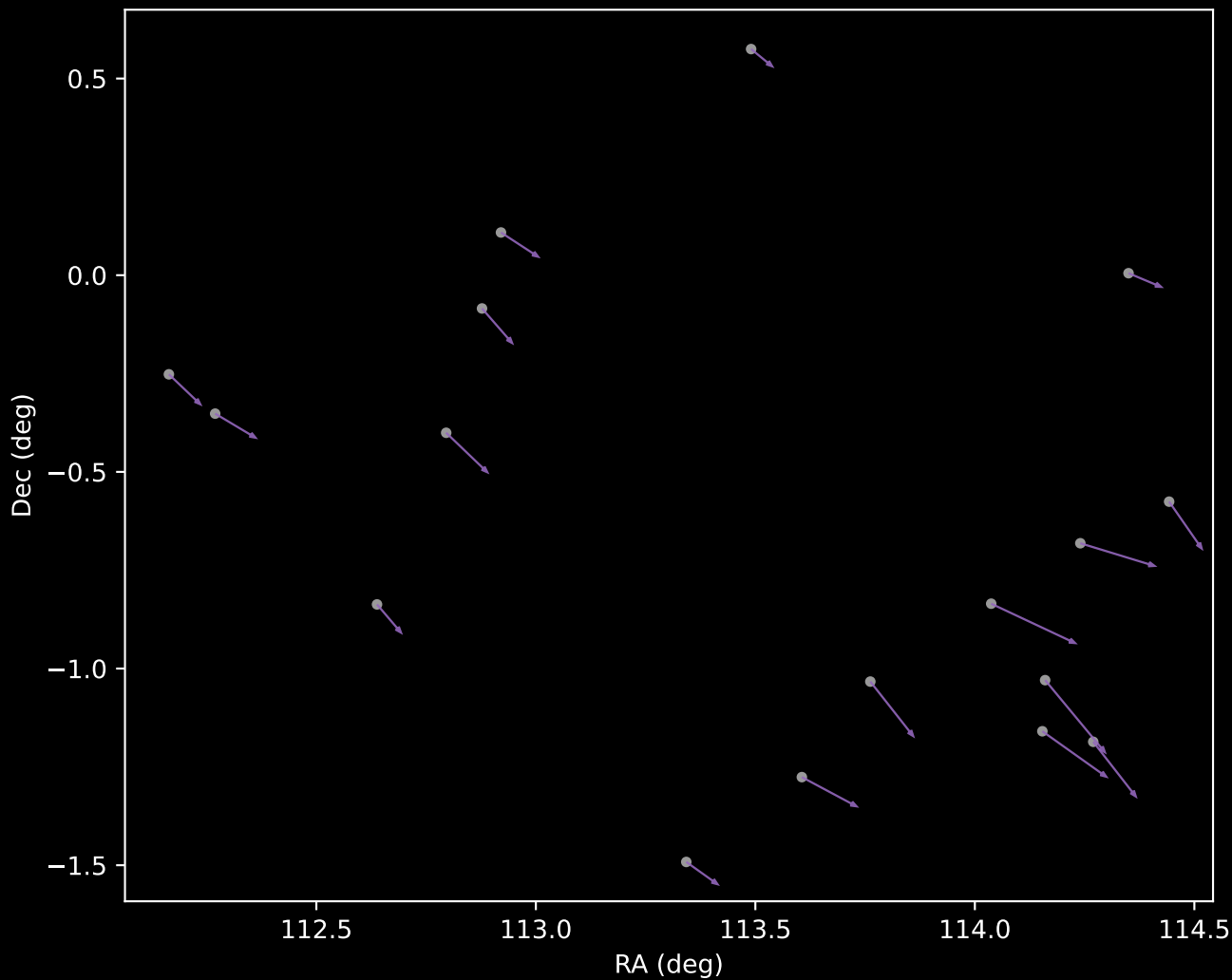
APOGEE DR17 Cluster 8 Proper Motion Vectors (n=17)
