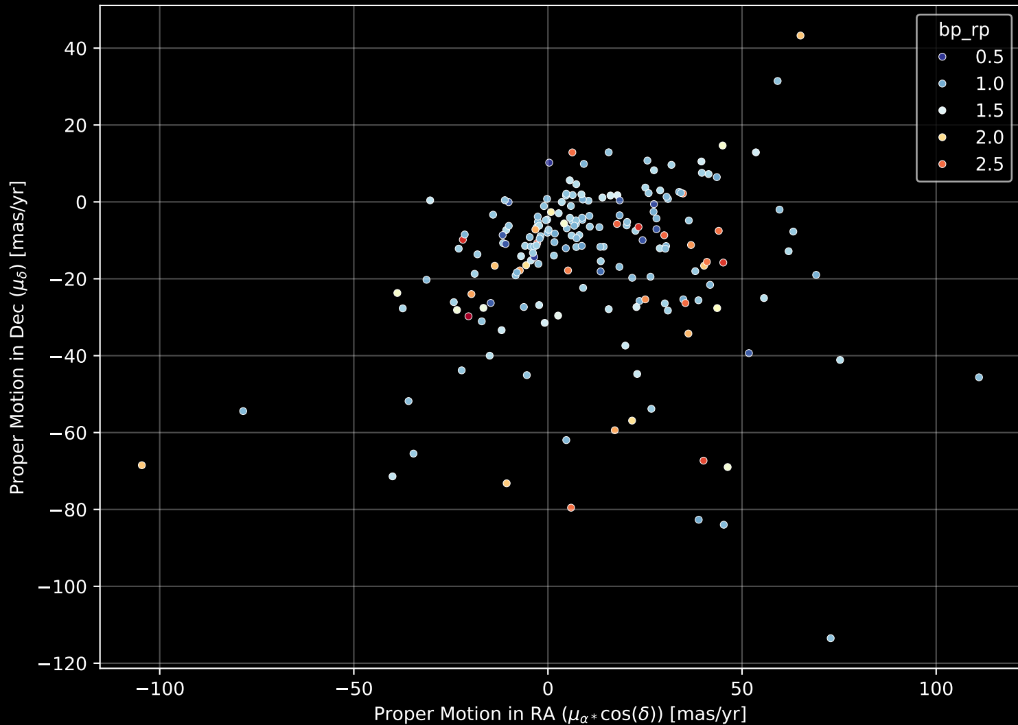
APOGEE DR17 Field: [K2_C8_124-63_btx] Proper Motion Diagram (n= 190)
